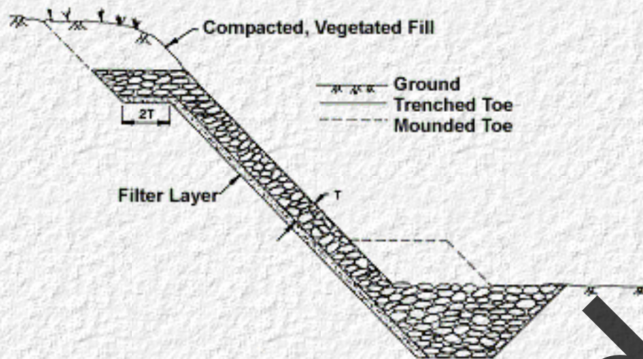
Figure 21. Typical Riprap Installation: End View (bank protection only)
