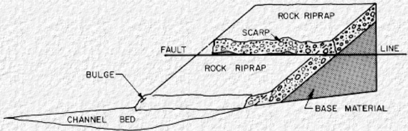
Figure 2. Translational Slide Failure (Modified from Blodgett (6))
