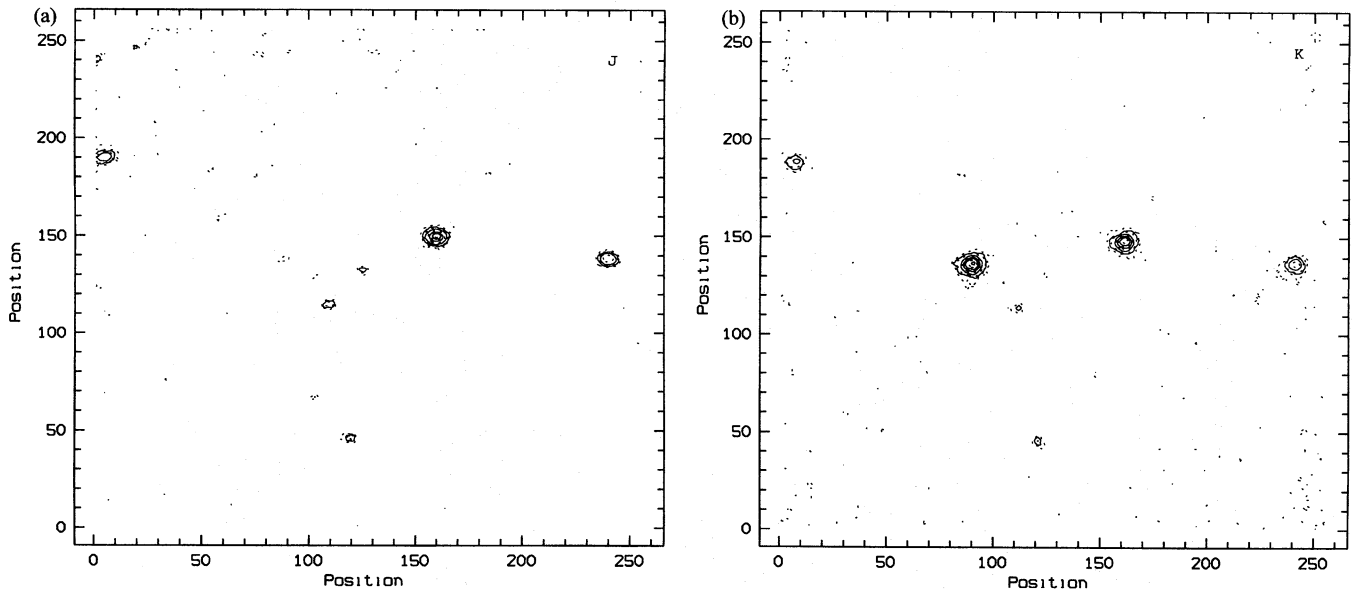
Figure 1. Contour plots of the area around 05329 – 6709 at J and K .
