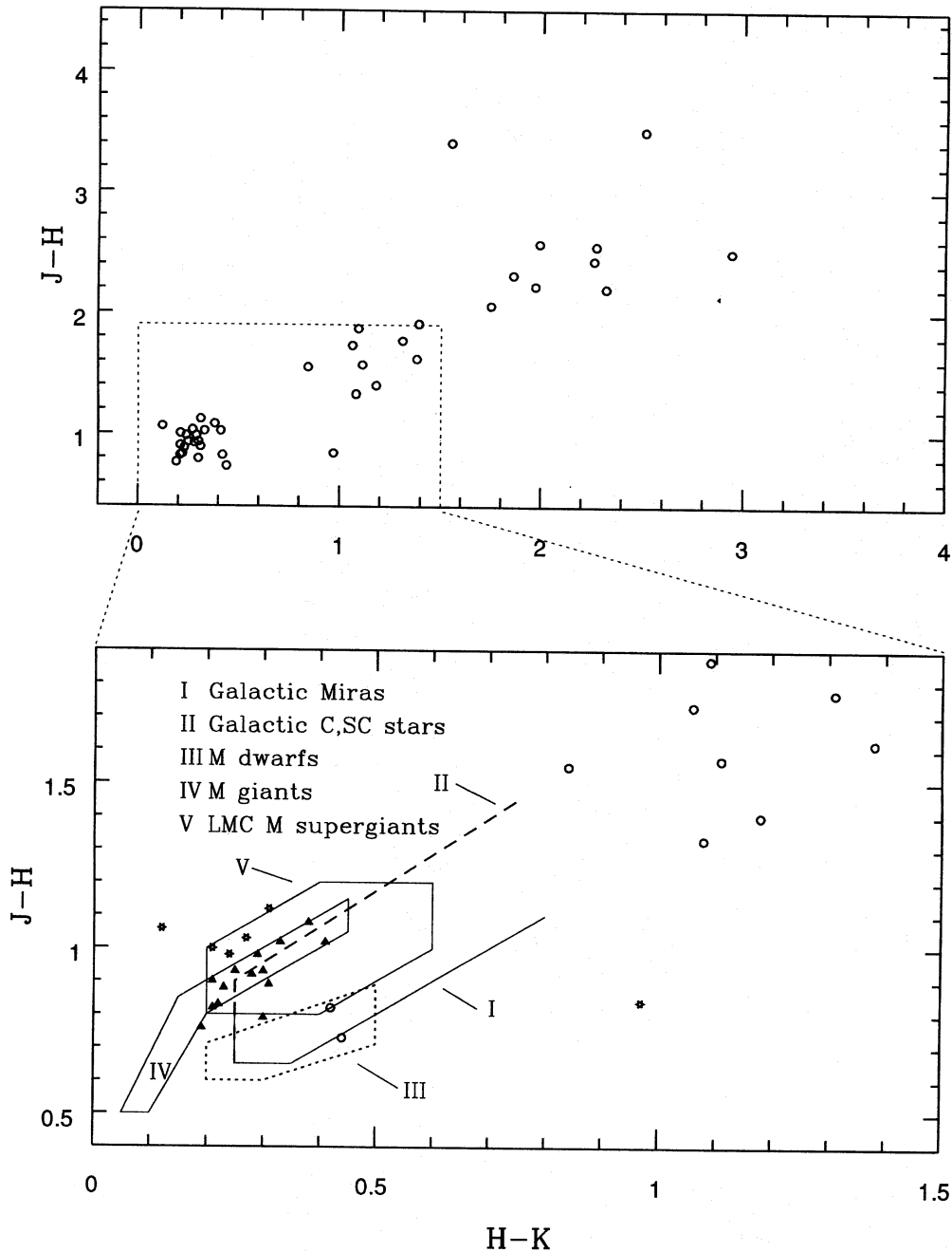
Figure 2. J-H versus H-K for the sources observed at ESO and SAAO. The lower diagram shows an enlargement of the bottom-left corner, indicating where various classes of stars would fall. In the lower diagram, the open circles indicate possible reddened AGB stars, the filled triangles possible M giants or supergiants, and the open star symbols foreground stars.
