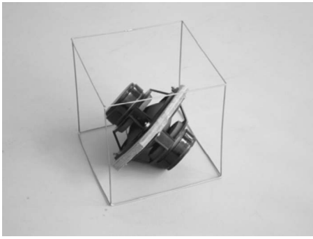
FIG. 9. Dipole source inside a very small measurement surface.
