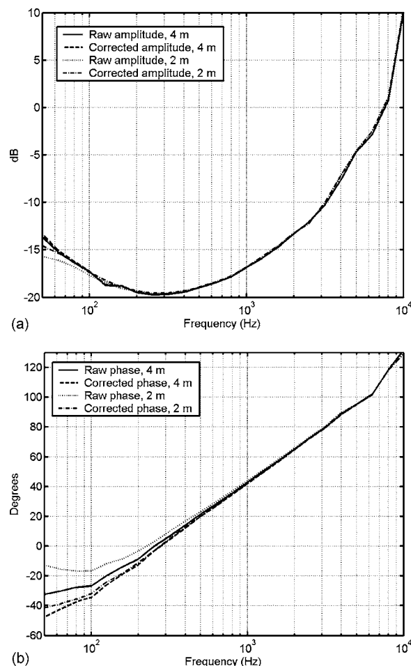
FIG. 3. Amplitude (a) and phase (b) calibration of the velocity signal relative to the pressure signal, measured at 2 and 4 m distance in an anechoic room, with and without correction for the finite distance to the loudspeaker.
