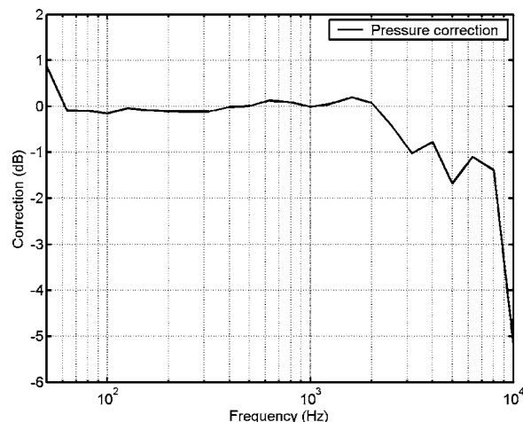
FIG. 4. Pressure correction of the MF probe.
