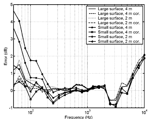
FIG. 8. Estimation error of the MF probe using different phase calibrations. A measurement with a BK intensity probe on the large measurement surface is used as the reference.
